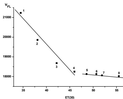
Fig. 3. Energy of the fluorescent maxima \nu_{FL} in \text{cm}^{-1} of compound 5 vs the solvent polarity parameter ET(30) in: benzene - 1; ethylacetate - 2; acetone - 3; acetonitrile - 4; n -buthanol - 5; i -propanol - 6; ethanol - 7; methanol - 8.
