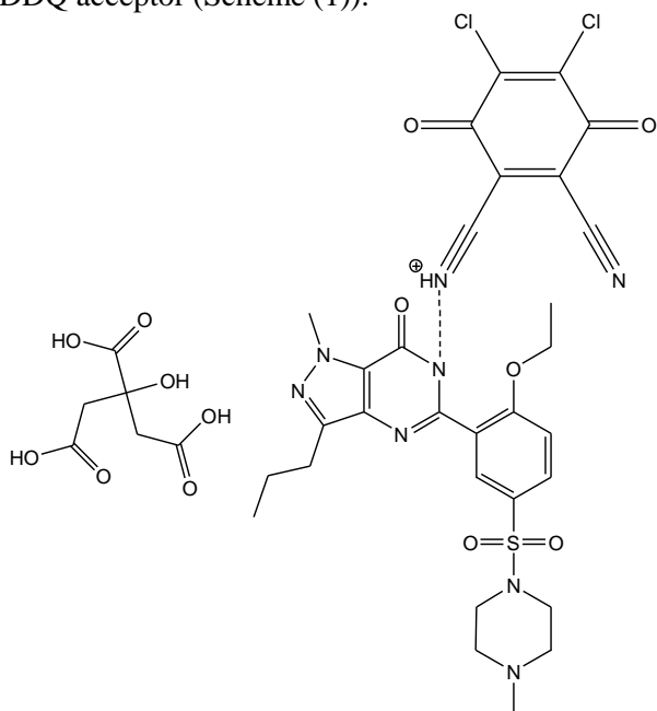
Scheme (1). Structure of the SILC-DDQ CT-complex.
