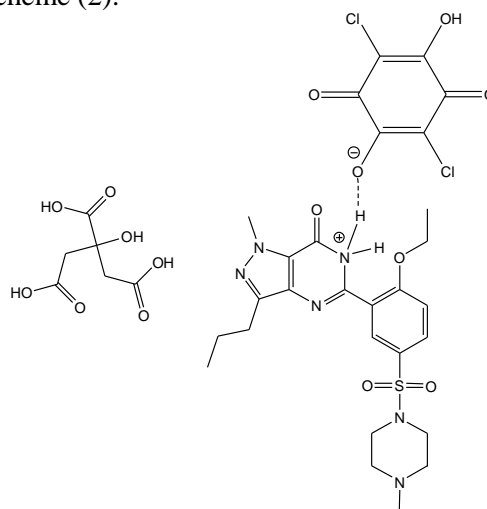
Scheme (2). Structure of the SILC-p-CLA CT-complex.
