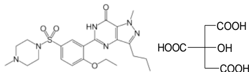
Scheme 1. Structure of sildenafil citrate.
