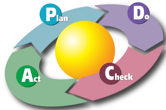
Fig. 4. PDCA Cycle [37].
