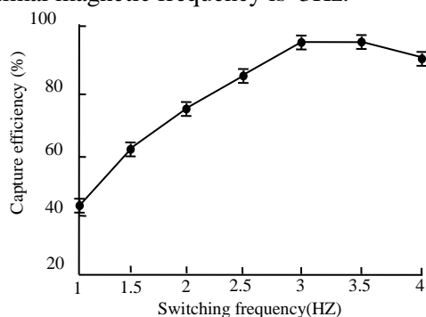
Fig.5. Capture efficiency VS. switching frequency.
