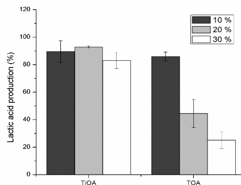
Figure 4. Lactic acid production for TiOA/dodecane and TOA/dodecane mixtures at three proportions of the tertiary amine.
