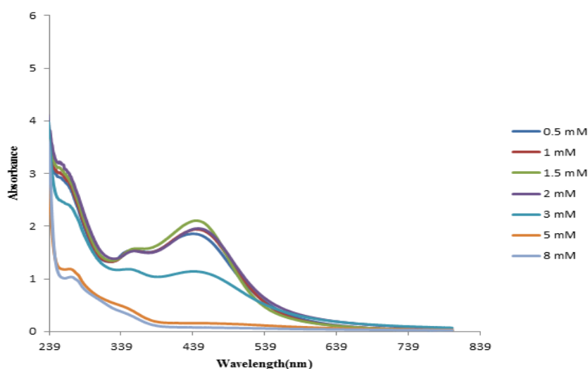
Figure. 5. Influence of silver nitrate concentration on silver nanoparticles synthesis. (Extract=2 \mu\text{l} , t=40\text{min} , T=\text{room} temperature, 150 rpm)
