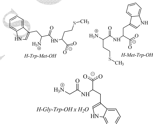
Scheme 1. Chemical diagram of dipeptides H-Trp-Met-OH , H-Met-Trp-OH and H-Gly-Trp-OH.2H 2 O .
