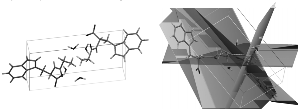
Scheme 4. Unit cell of H-Gly-Trp-OH.2H 2 O .
