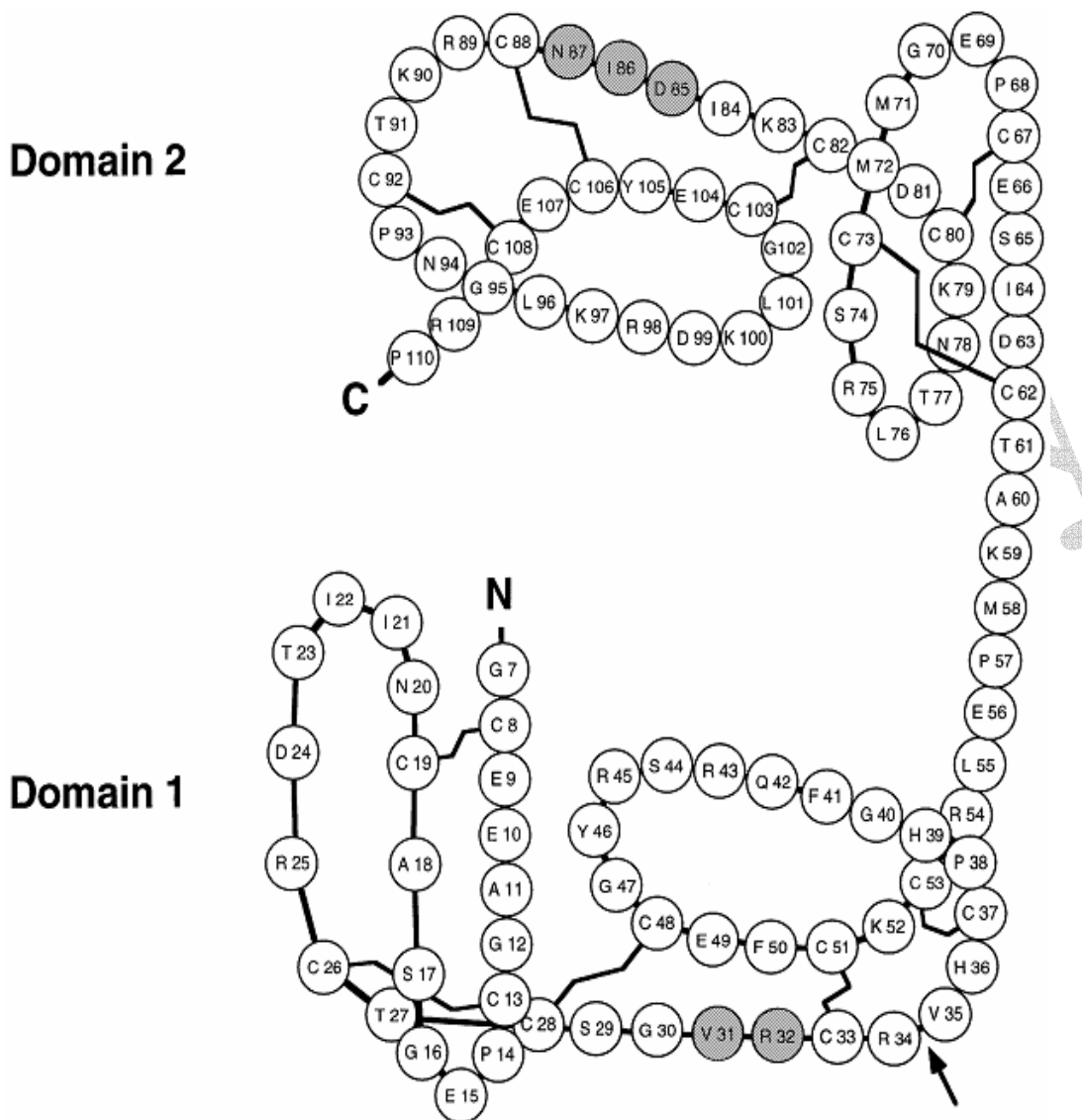
Fig. 2. Primary structure of antistasin.
