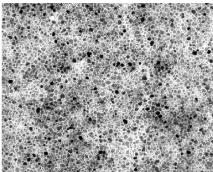
Figure 3. TEM image of \text{CoFe}_2\text{O}_4 nanoparticles.
