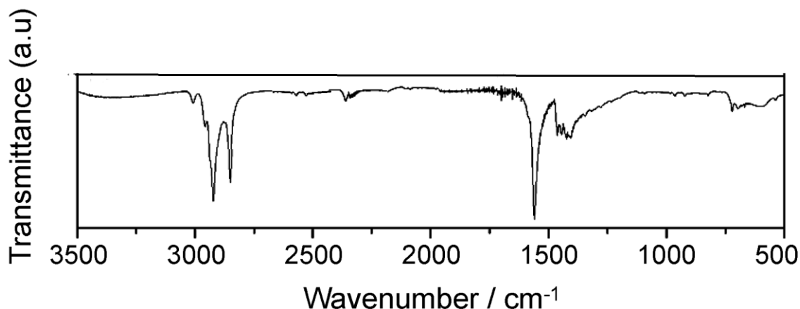
Fig. 2. FT-IR spectra \text{CoFe}_2\text{O}_4 nanoparticle coated with oleic acid.
