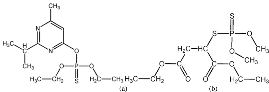
Fig. 1. Chemical structure of (a) Diazinon (b) Fenitrothion.
