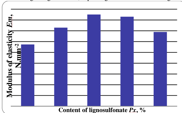
Figure 2. Modulus of elasticity in bending of MDF, depending on the content of the lignosulphonate.
