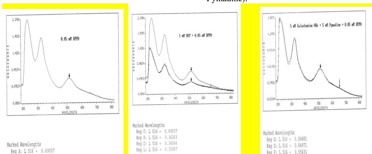
Figure 5. Spectra of 0.05 mM solution of DPPH-radical: A 0 min. = 0.69037 and after 30 min reaction with 1 mM BHT and 5 mM Galantamine hydrobromide/5 mM Pymadine.
