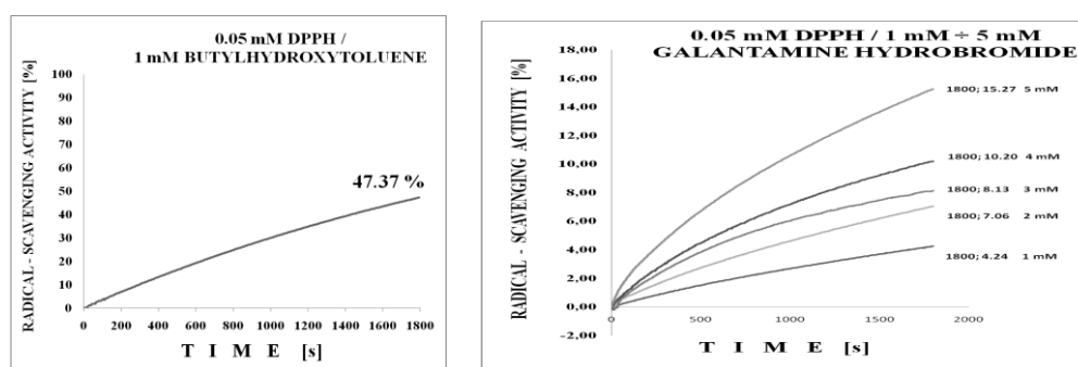
Figure 2. Kinetics of scavenging of 0.05 mM DPPH-radical from 1 mM BHT and 1 mM ÷ 5 mM Galantamine hydrobromide for a period of 30 min.
