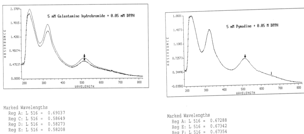
Figure 6. Spectra of 0.05 mM solution of DPPH-radical after 30 min. interaction with 5 mM Galantamine hydrobromide and 5 mM Pymadine.
