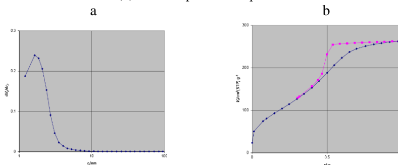
Fig. 7. (a) BJH pore size distribution and (b) N 2 adsorption-desorption isotherm heat treated at 600 °C.
