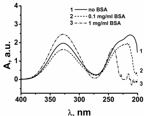
Fig. 1. UV spectra of HAOA: alone (1), in the presence of 0.1 mg/ml BSA (2) and in the presence of 1 mg/ml BSA (3).
