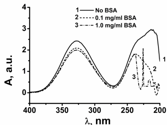
Fig. 2. UV spectra of PrAOA: alone (1), in the presence of 0.1 mg/ml BSA (2) and in the presence of 1 mg/ml BSA (3).
